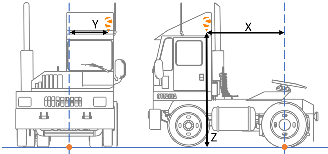
Figure 2-7: The location of the constraint point (orange dot) and the receiver (Septentrio logo) in the vehicle. Front view on the left, side view on the right.
